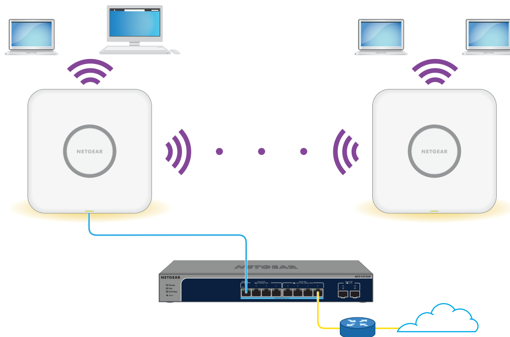
Figure 8. WiFi bridge configuration between two APs in the 5 GHz radio band
