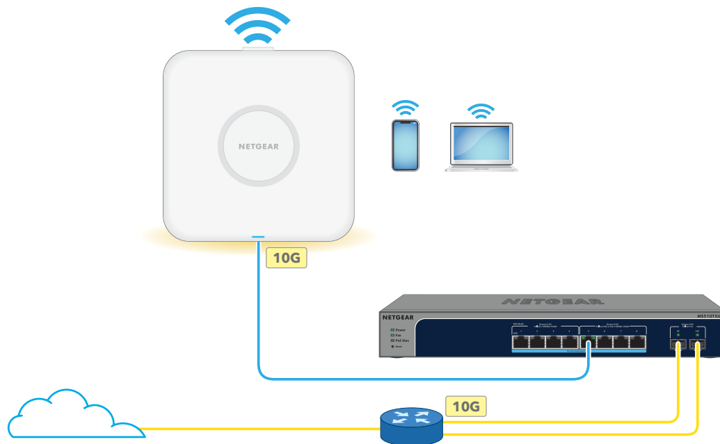
Figure 4. Set up the AP with a PoE++ connection to your network
