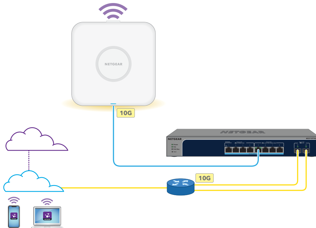
Figure 5. Set up the AP in a NETGEAR Insight configuration
