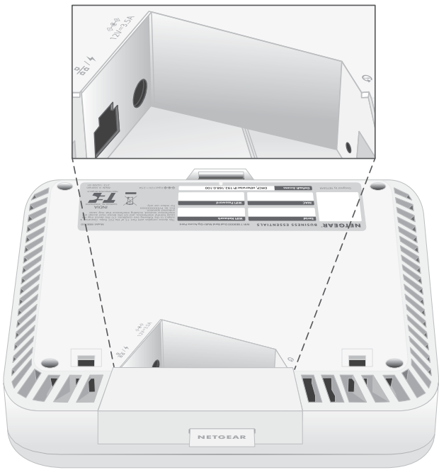
Figure 2. Hardware interfaces
