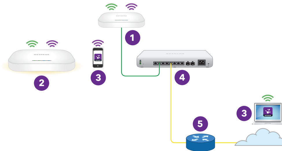
Figure 9. Mesh network with a node and a wired root
