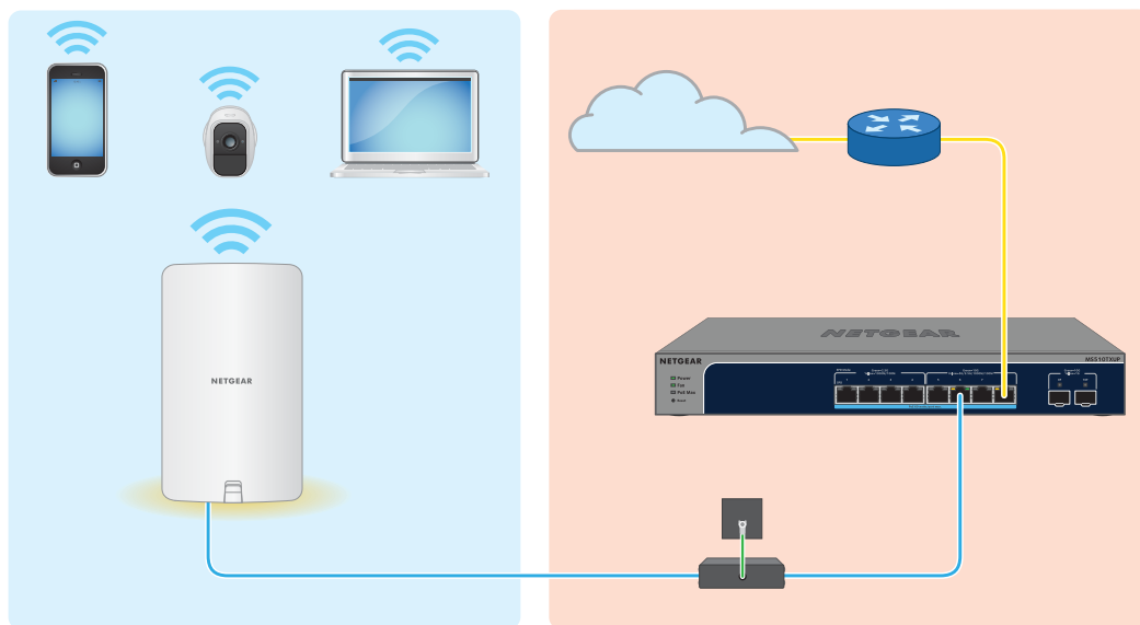
Figure 8. Set up model WAX610Y with a PoE+ connection to your network
