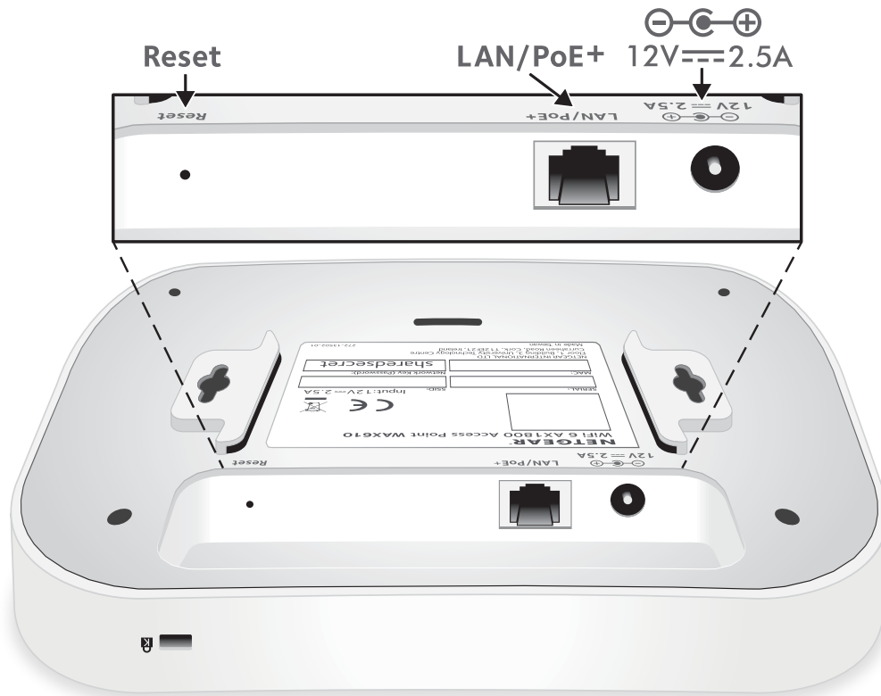
Figure 2. Hardware interfaces of indoor model WAX610
