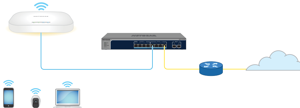
Figure 7. Set up model WAX610 with a PoE+ connection to your network
