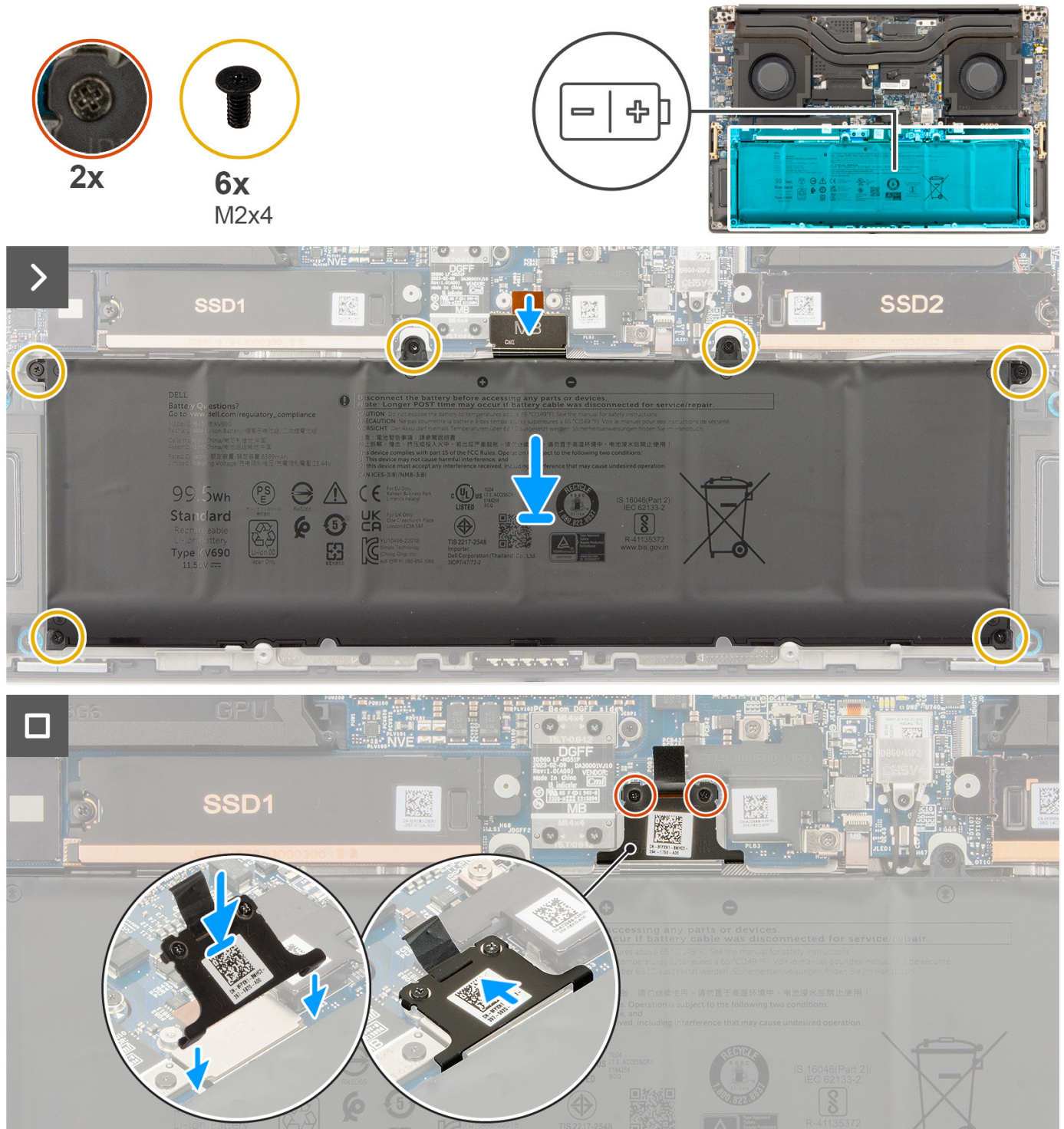
Figure 21. Installing the battery
