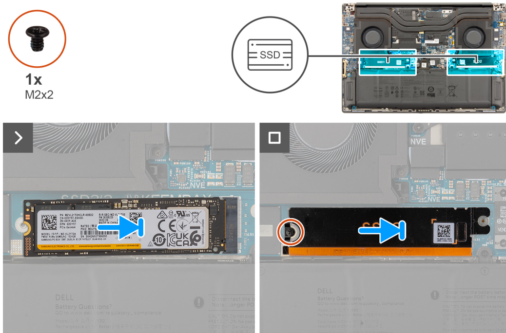
Figure 19. Installing the M.2 2280 SSD
