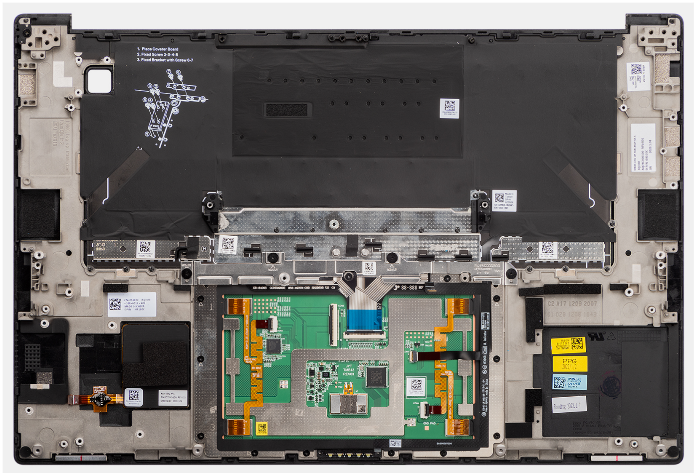
Figure 82. Installing the palm-rest and keyboard assembly
